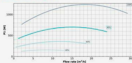
POWER CONSUMPTION 1.5 HP
