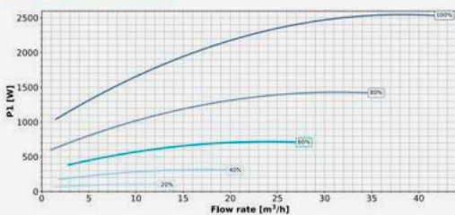
POWER CONSUMPTION 3 HP
