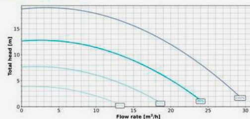
PERFORMANCE 1.5 HP
