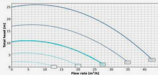
PERFORMANCE 3 HP
